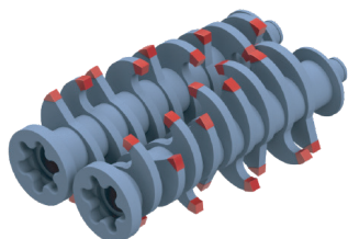
CONCRETE SHAFTS
